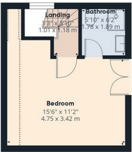
Floor 2 Building 1
